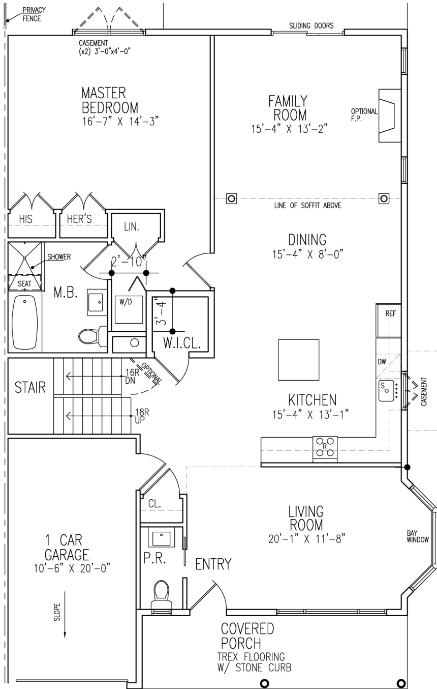
First Floor, 1442 Square Feet
